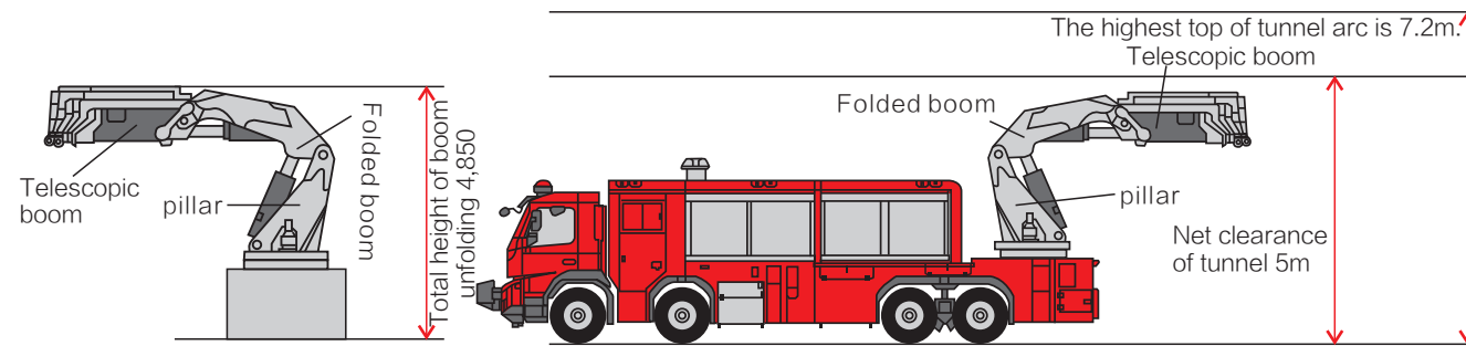
Small boom unfolding space
